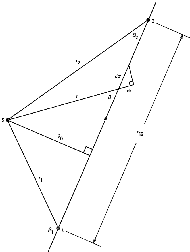
Fig. C-1. Geometry for straight line motion
