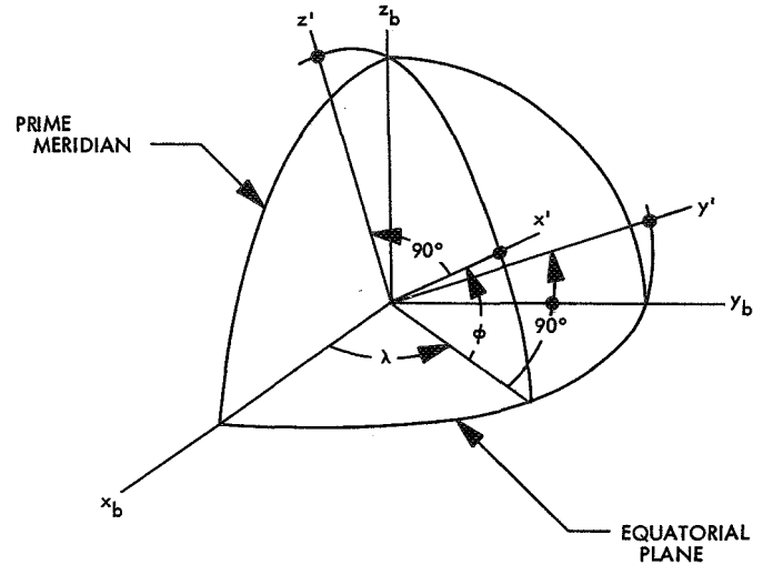
Fig. 3. x' , y' , and z' axes relative to body-fixed x_b , y_b , and z_b axes
