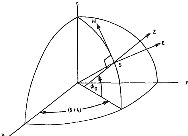
Fig. 6. The north-east-zenith coordinate system
