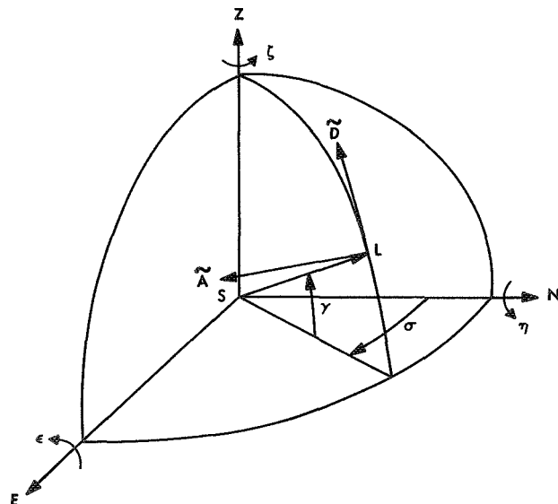
Fig. 7. Azimuth and elevation
