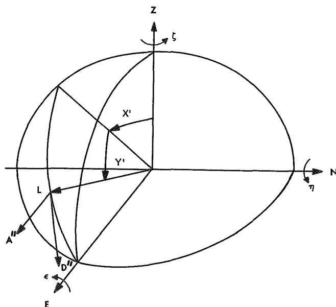
Fig. 9. X' and Y' angles
