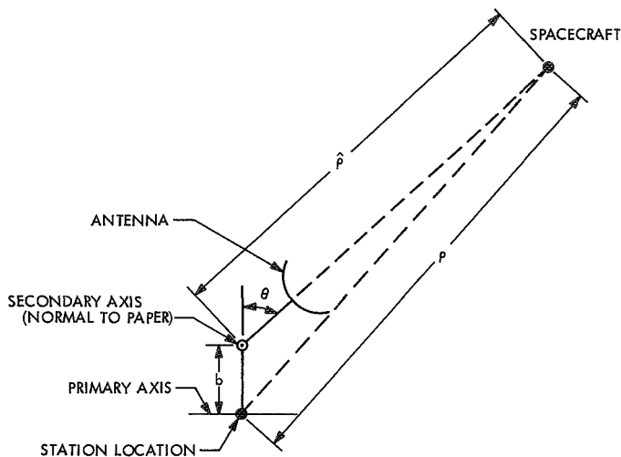
Fig. 10. Antenna correction
