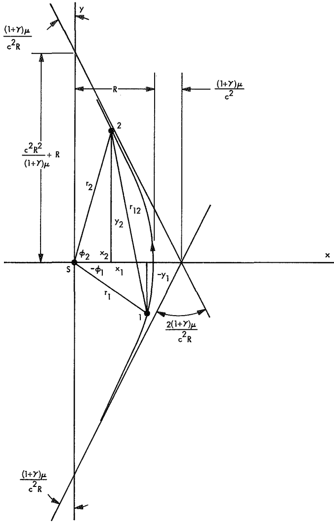
Fig. 2. Light path
