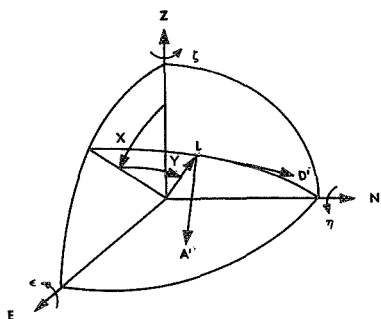
Fig. 8. X and Y angles
